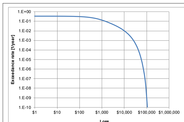
FIGURE 1. Schematic LEC
