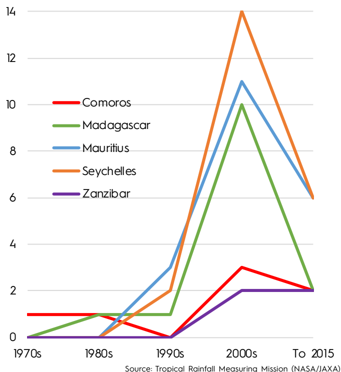
Number of recorded non-cyclone flooding events for each SWIO island nation, by decade
